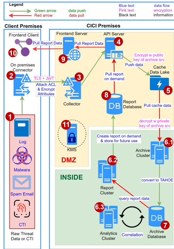
Figure 1.2: System architecture diagram for the CYBEX-P platform.
