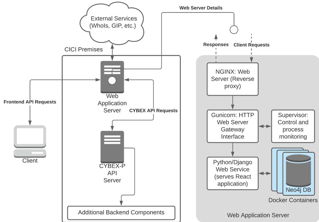
Figure 1.3: High-level architectural diagram for the CYBEX-P web application.
