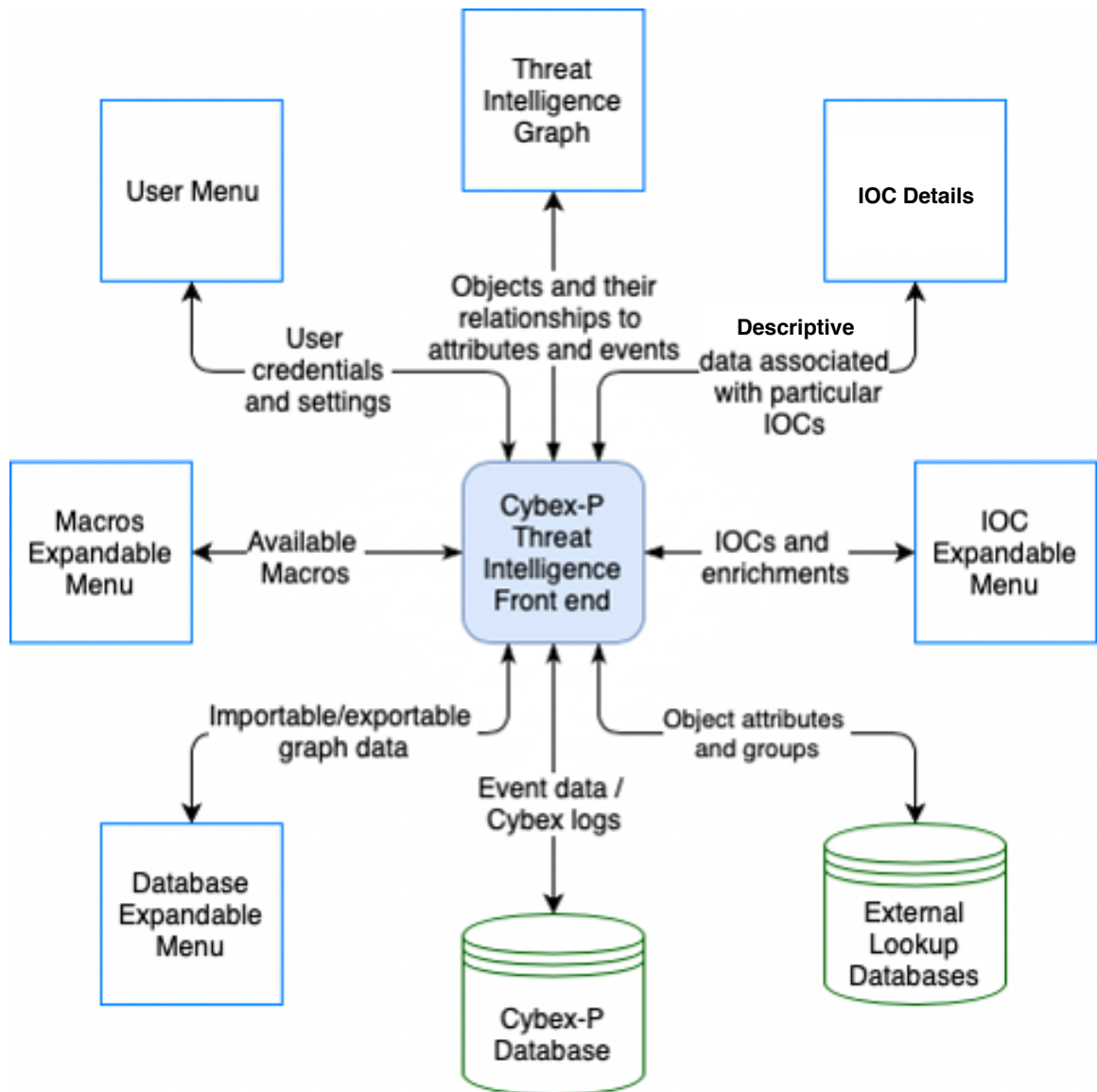
Figure 1.1: System context diagram illustrating the high-level structure of some of the application's interactions.
